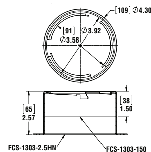
FCS-1303-2.5HN FCS-1303-150
