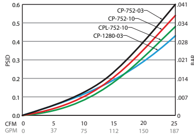
LGB Series Performance Graphs
